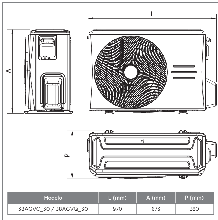
FIG. 5 - DIMENSIONAL
