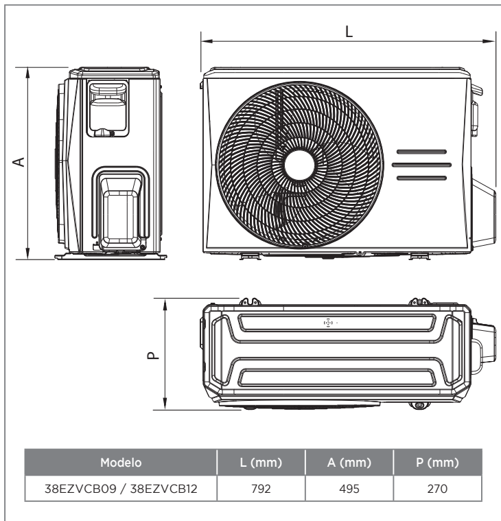
FIG. 4 - DIMENSIONAL
