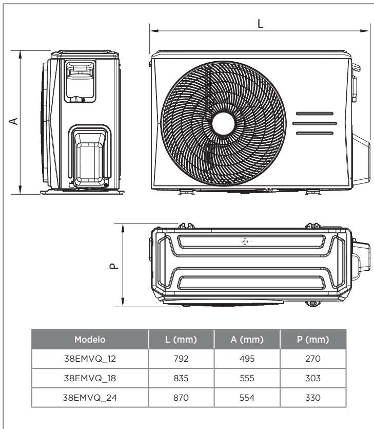
FIG. 4 - DIMENSIONAL
